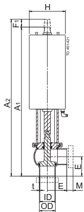
Shut-off valve.
