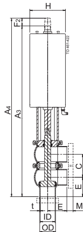
Change-over valve.
